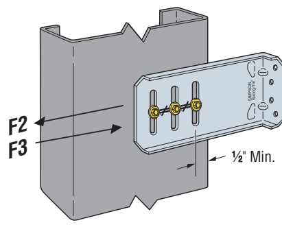
SCB Installation with 3 Shouldered Screws
