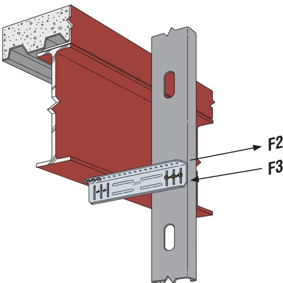
Typical SSB3.518 Installation
