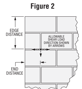
Figure 2 Anchor placement in grouted CMU mortar "T" joint
