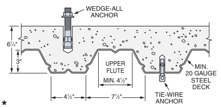
Lightweight Concrete On Metal Deck
