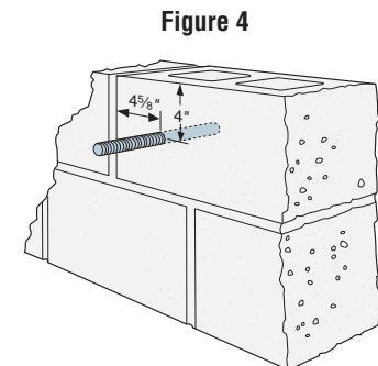
Figure 4 Anchor installed in face shell w/ screen tube in hollow cell
