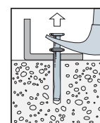
Duplex-head anchor may be removed with a claw hammer
