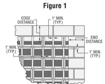
Figure 1 Allowable anchor placement in grouted CMU face shell
