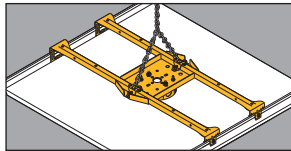
Figure 32 - BA50F
